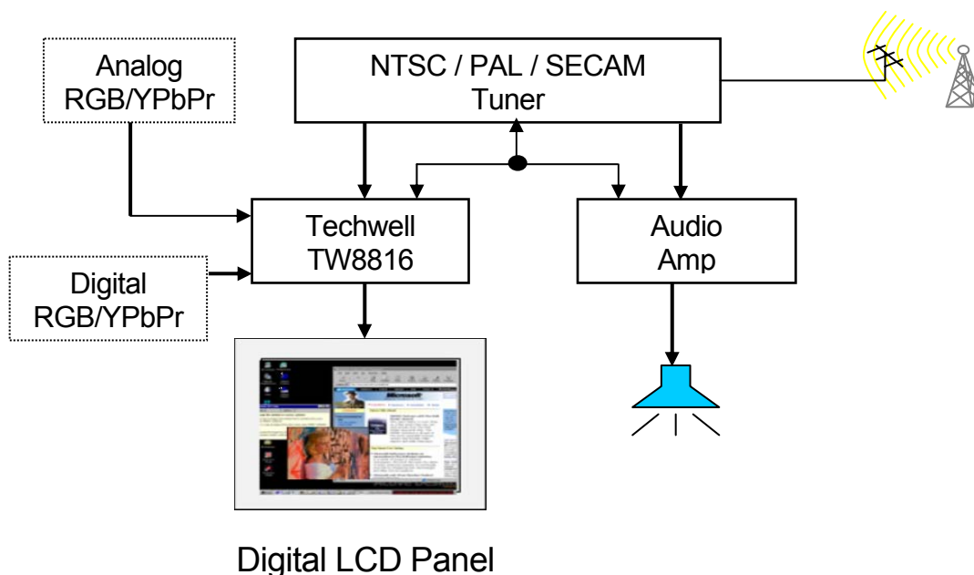
Figure 2 TW8816 Flat Panel TV/Monitor controller system block diagram
