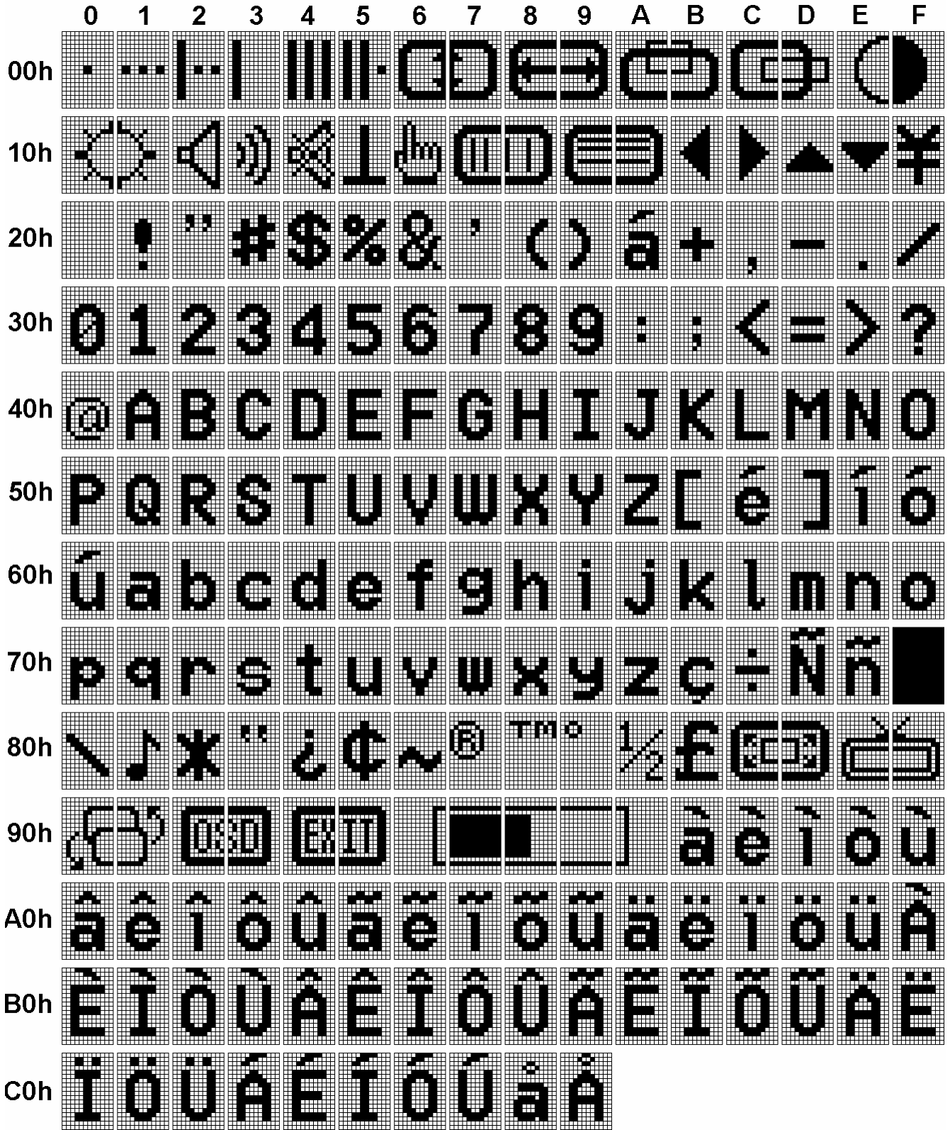
Figure 4 Font ROM Characters and Addresses
