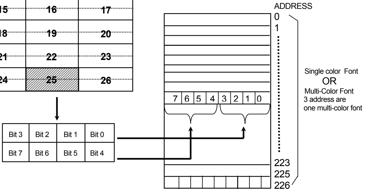
FONT RAM (6144 x 8 bits)
